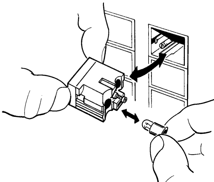
DUAL LAMP ASSEMBLY
