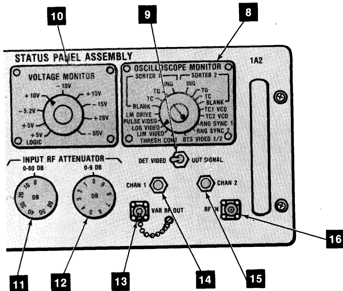
RIGHT HALF OF STATUS PANEL ASSEMBLY, CONTROLS AND INDICATORS
